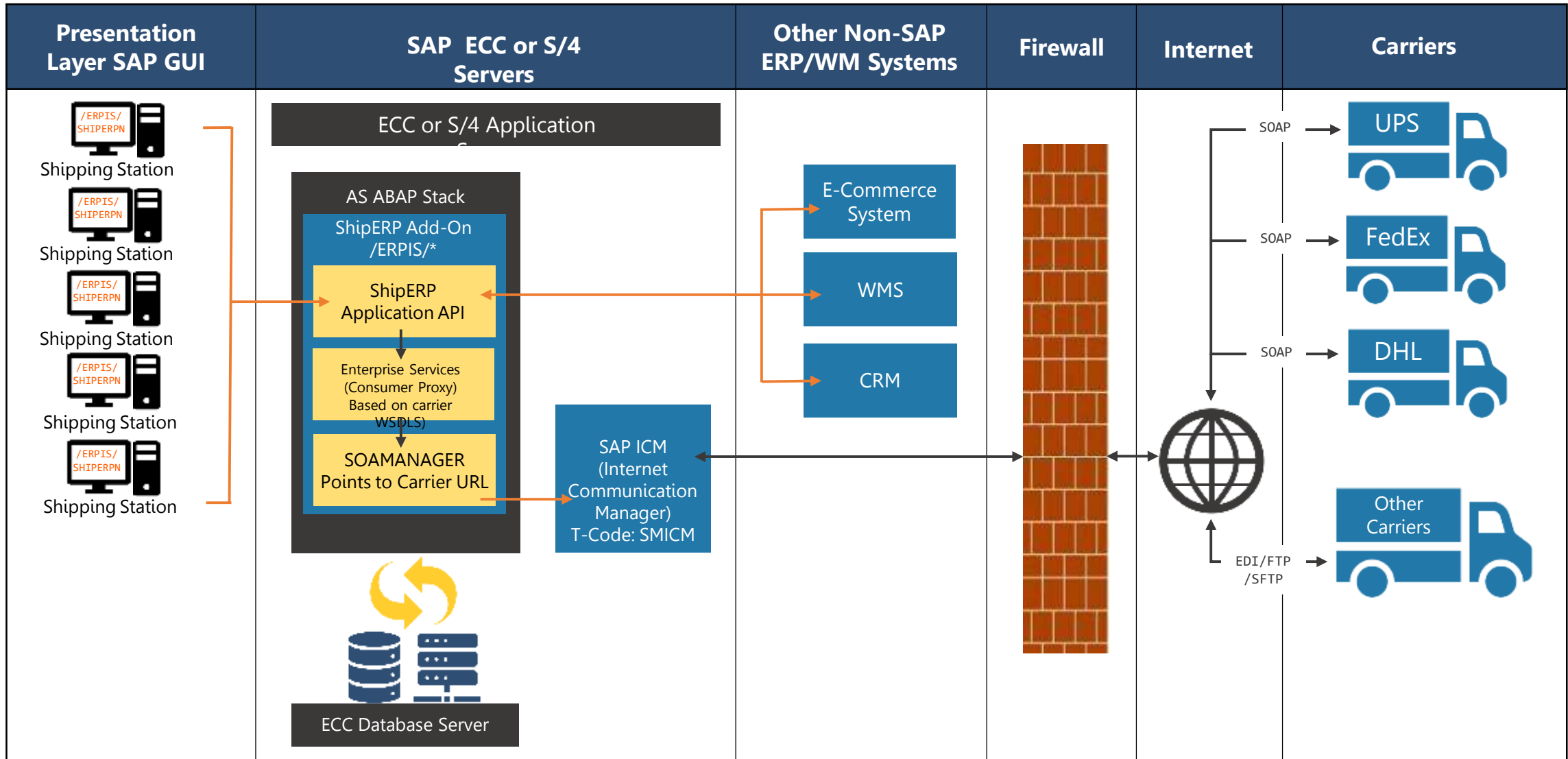
ShipERP – Network Communication with Carriers – Topology – External Systems
